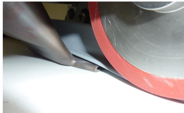
Adjust nozzle centered on structural profile
